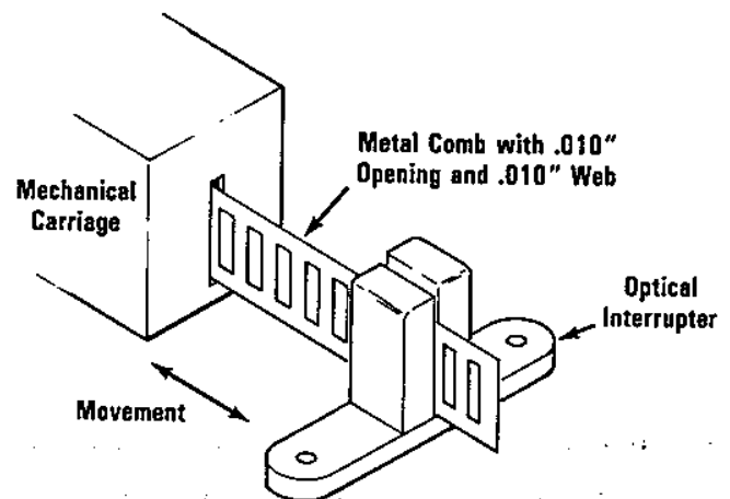
Figure 2 - Linear Encoder Relating Distance Versus Pulses
