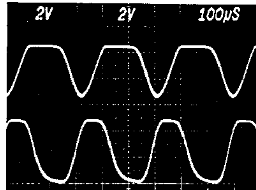
Figure 6 - OPB860T55 (upper) Versus OPB860T51 (lower)
