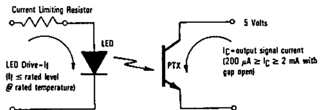
Figure 3 - Schematic/Drive
