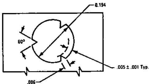
Figure 8 - Tightening Ribs
