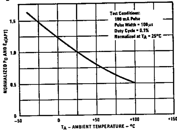
Figure 13 - Normalized P D and E a (APT) vs. Ambient Temperature
