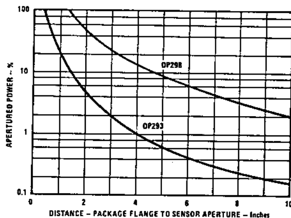
Figure 12 - Normalized Power vs. Distance
