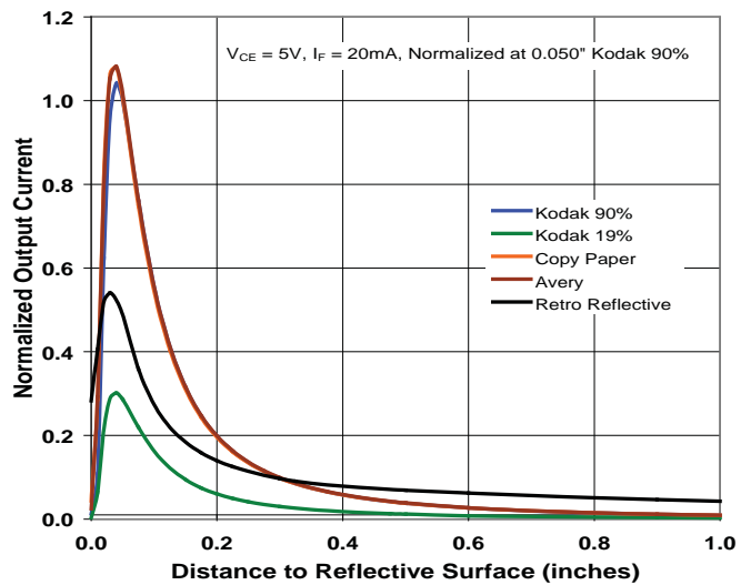
Graph of OPB706 Unfocused Normalized Collector Current vs. Distance Reflective Surface.
