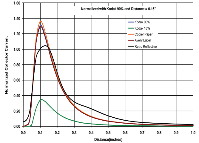
Graph of OPB700 Focused Normalized Collector Current vs. Distance to a Reflective Surface.
